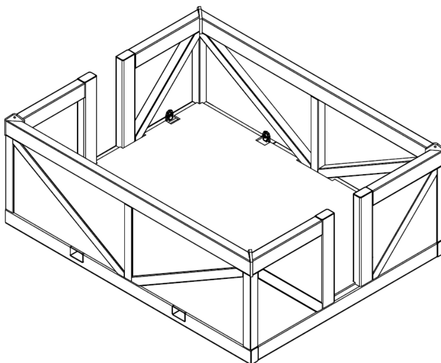
ISOMETRIC VIEW
